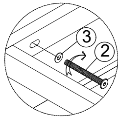
DETAIL T-T
